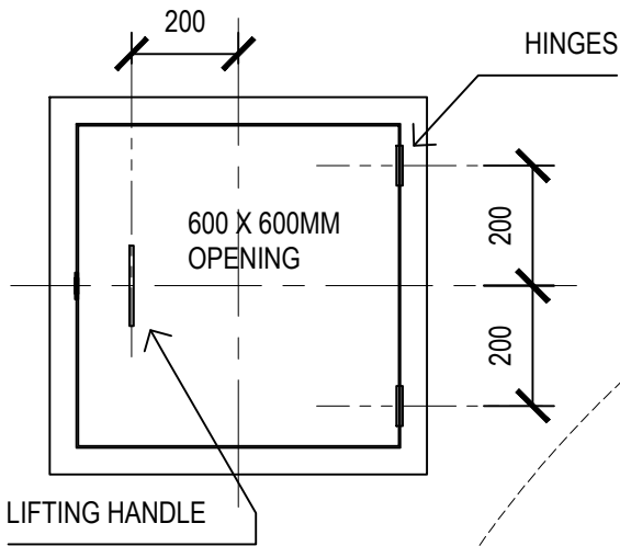
MANHOLE COVER PLAN SCALE 1:16
